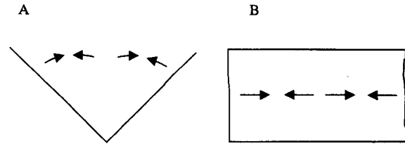
Figure 1. Schematic of biases in remembered location. A: The V frame task from Engebretson and Huttenlocher (1996). B: The rectangular frame task from Huttenlocher, Newcombe, and Sandberg (1994). Lines with arrows show direction of systematic biases in constant (mean) error. Panel A is from “Bias in Spatial Location Due to Categorization: Comment on Tversky and Schiano,” by P. H. Engebretson and J. Huttenlocher, 1996, Journal of Experimental Psychology: General , 125, p. 97. Copyright 1996 by the American Psychological Association. Adapted with permission of the author. Panel B is from “The Coding of Spatial Location in Young Children,” by J. Huttenlocher, N. Newcombe, and E. H. Sandberg, 1994, Cognitive Psychology , 27, p. 126. Copyright 1994 by Academic Press. Adapted with permission.
