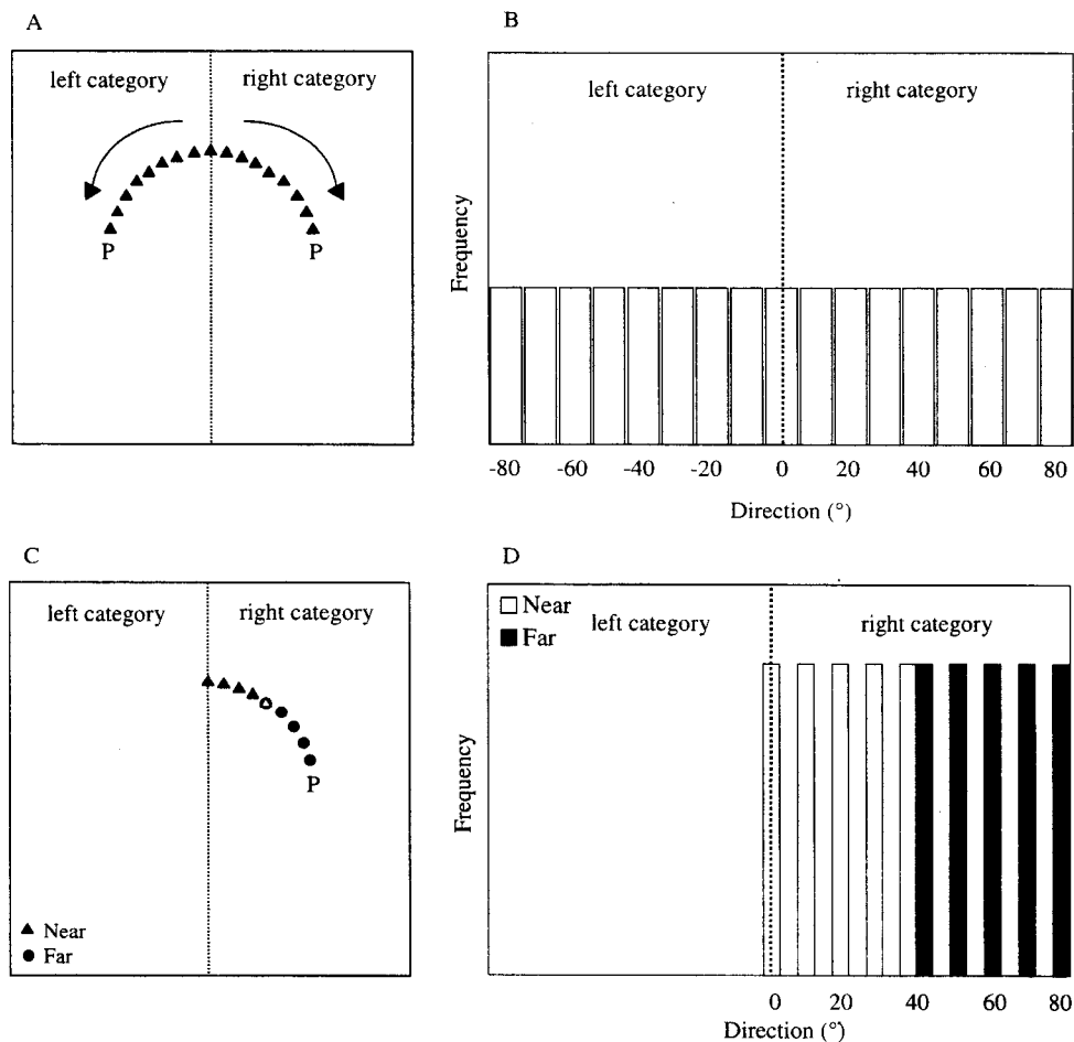
Figure 3. A and B: Target locations and frequency distribution of target presentation from a hypothetical experiment similar to that of Engebretson and Huttenlocher (1996). The dotted lines illustrate the midline axis, which divides the task space into two categories (left and right). Geometric prototypes are marked by P s. Lines with arrows in Panel A show the direction of systematic biases toward geometric prototypes at \pm 90^\circ . C and D: Target locations and associated frequency distribution for a hypothetical experiment investigating induced category effects. Triangles in Panel C represent targets in a “near” category; circles represent targets in a “far” category. White bars in Panel D depict target frequencies in the near condition; black bars depict target frequencies in the far condition.
