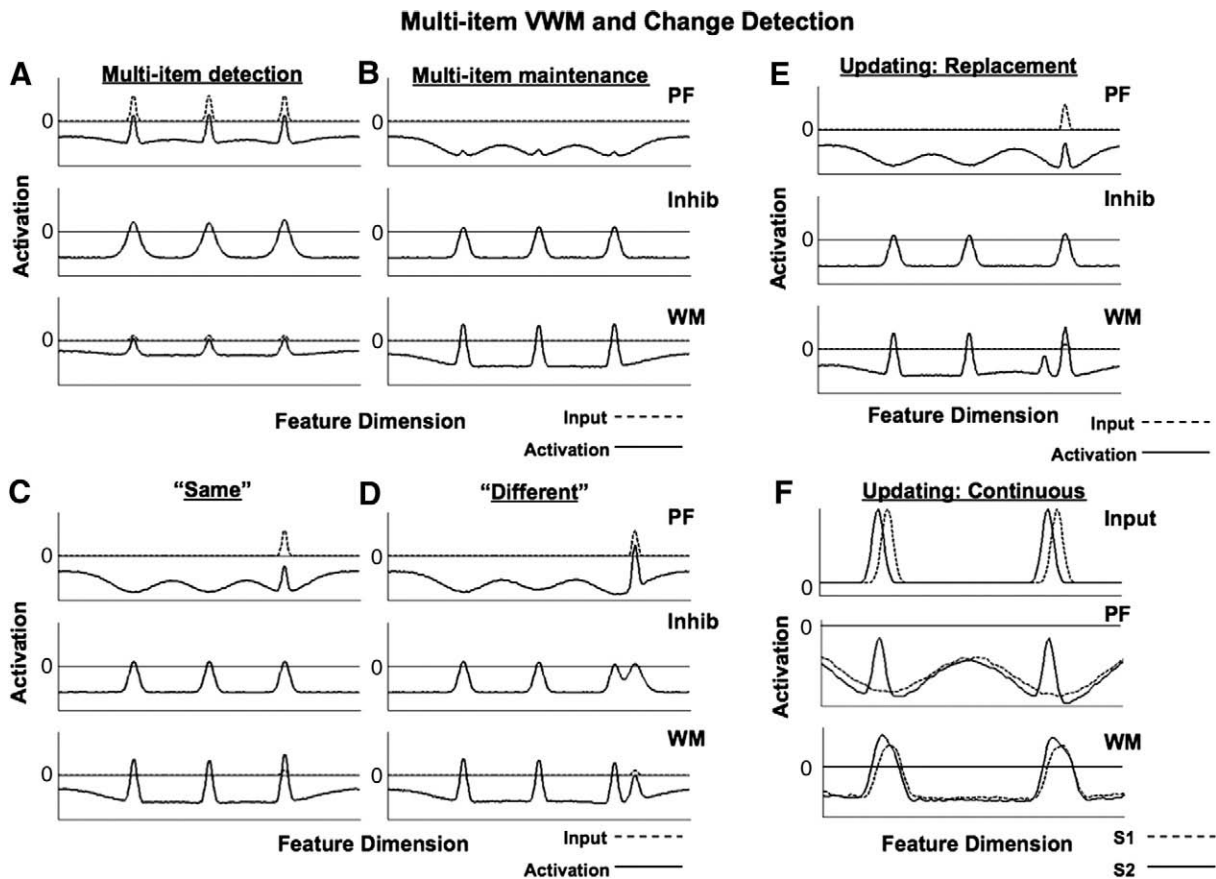
Fig. 6 – Simulations of the three-layer model in response to multiple simultaneous inputs. (A) and (B) show the detection of the inputs by PF, and their consolidation and maintenance in WM, respectively. The simulations in (C) and (D) show the generation of “same” and “different” responses in the multi-item case. Finally, (E) and (F) show two different forms of updating in the model. In the first case, the presentation of a changed input at test results in the destabilization of the original peak in WM and its replacement by the new value. In the second case (F), activation in WM is updated in a continuous fashion in response to new input. Note, that the scale of the simulations shown in (F) has been magnified, and the inputs to the model are now shown in the top panel. The first (S1) and second (S2) stimuli presented to the model are indicated by dashed and solid lines, respectively.
