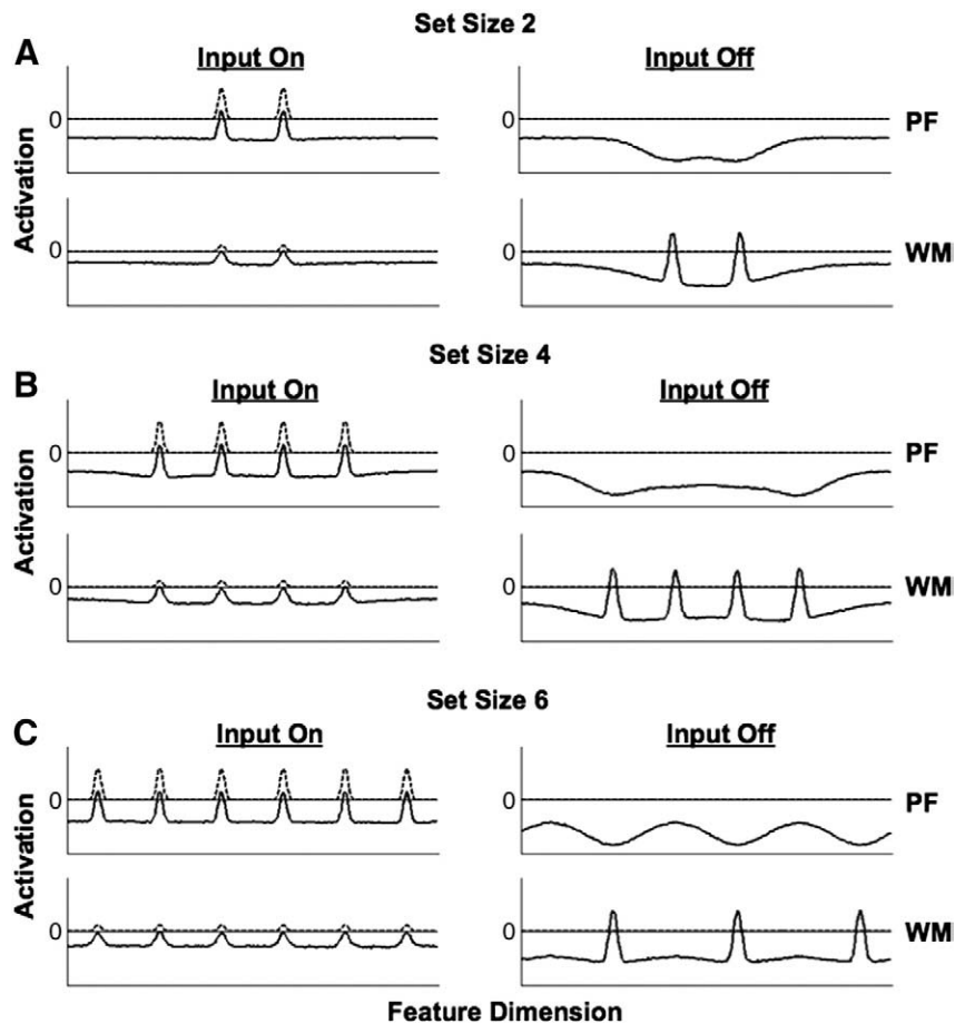
Fig. 7 – Simulations showing capacity limits in the three-layer neural field model. The simulations in (A) and (B) show the model successfully maintaining up to four peaks of activation simultaneously in WM. However, when two more items are added, inhibitory input to WM outweighs excitation, and three of the items failed to be sustained in the absence of input. Note that, for simplicity, the inhibitory layer is not shown here.
