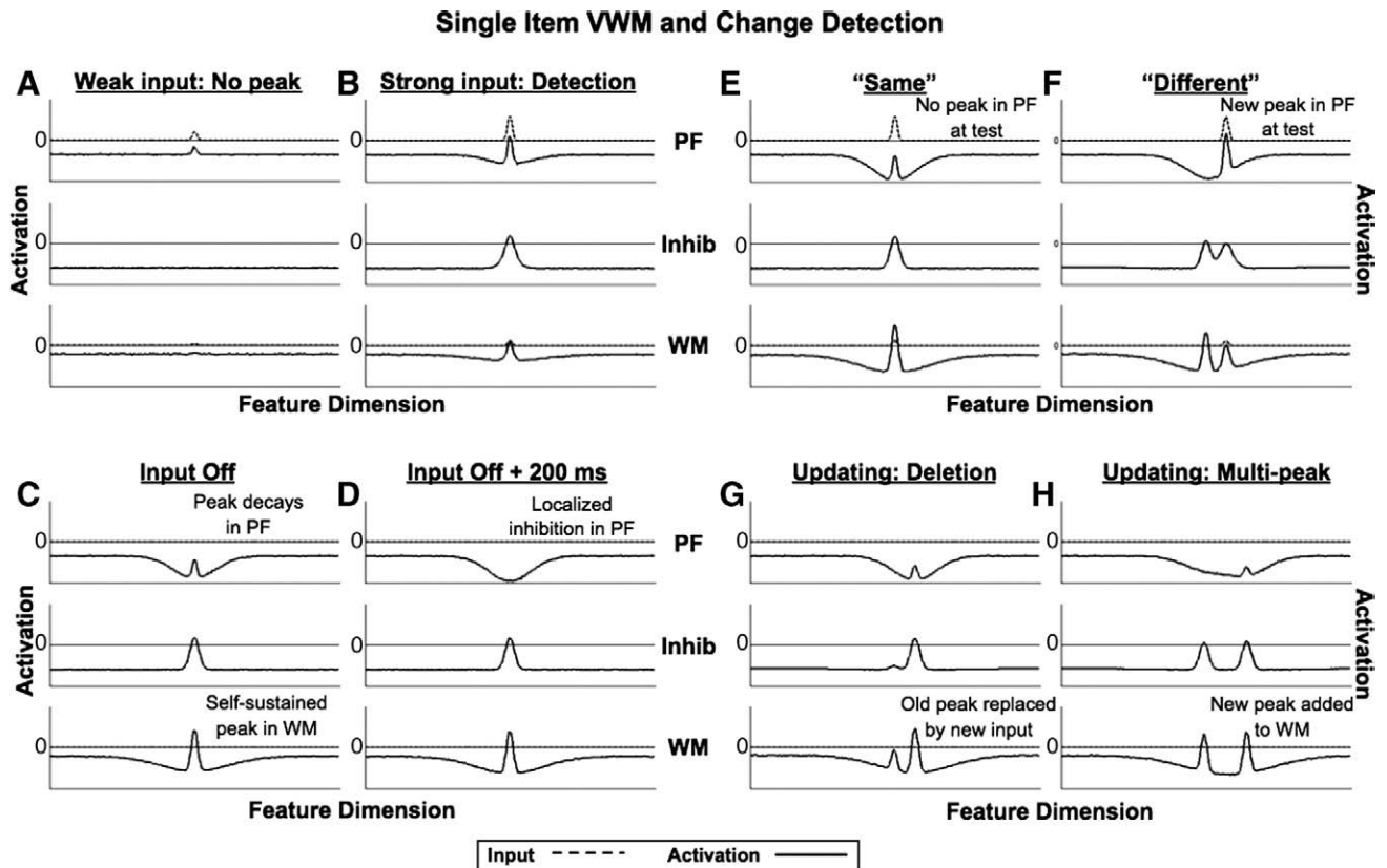
Fig. 5 – Simulations demonstrating the emergent functionality of the three-layer model in response to a single input.
